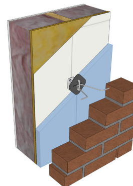
Brick ties
