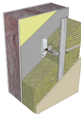
Proprietary aluminium clip
